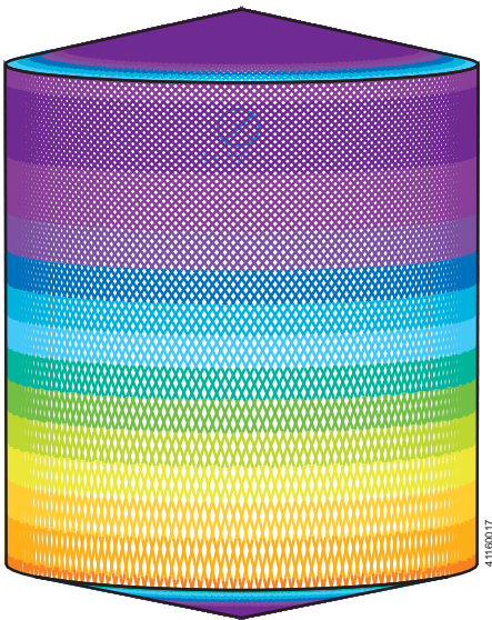
D4.6m H5.5m, Toftejorg TJ40G, 4 x ø7.3 mm, Time = 16 min., Water consumption = 5600 l
