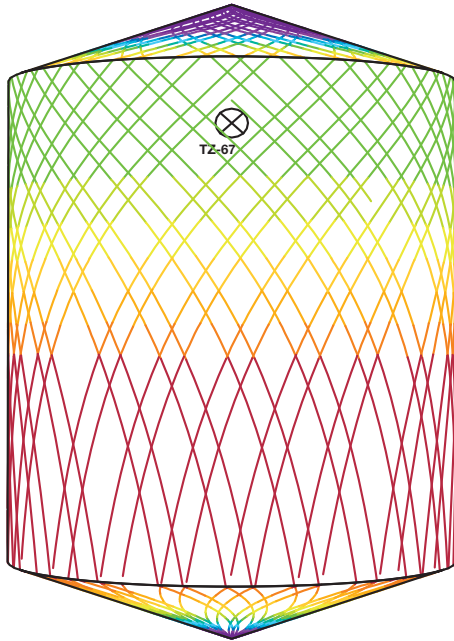
D2.5m H6m, Toftejorg TZ-67, 4 x \varnothing 6 mm Time = 3.5 min., Water consumption = 727 l
