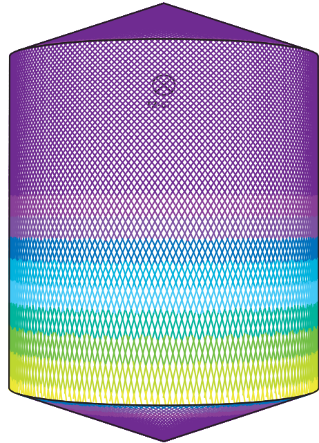
D2.5m H6m, Toftejorg TZ-67, 4 x \varnothing 6 mm Time = 14.7 min., Water consumption = 3097 l
